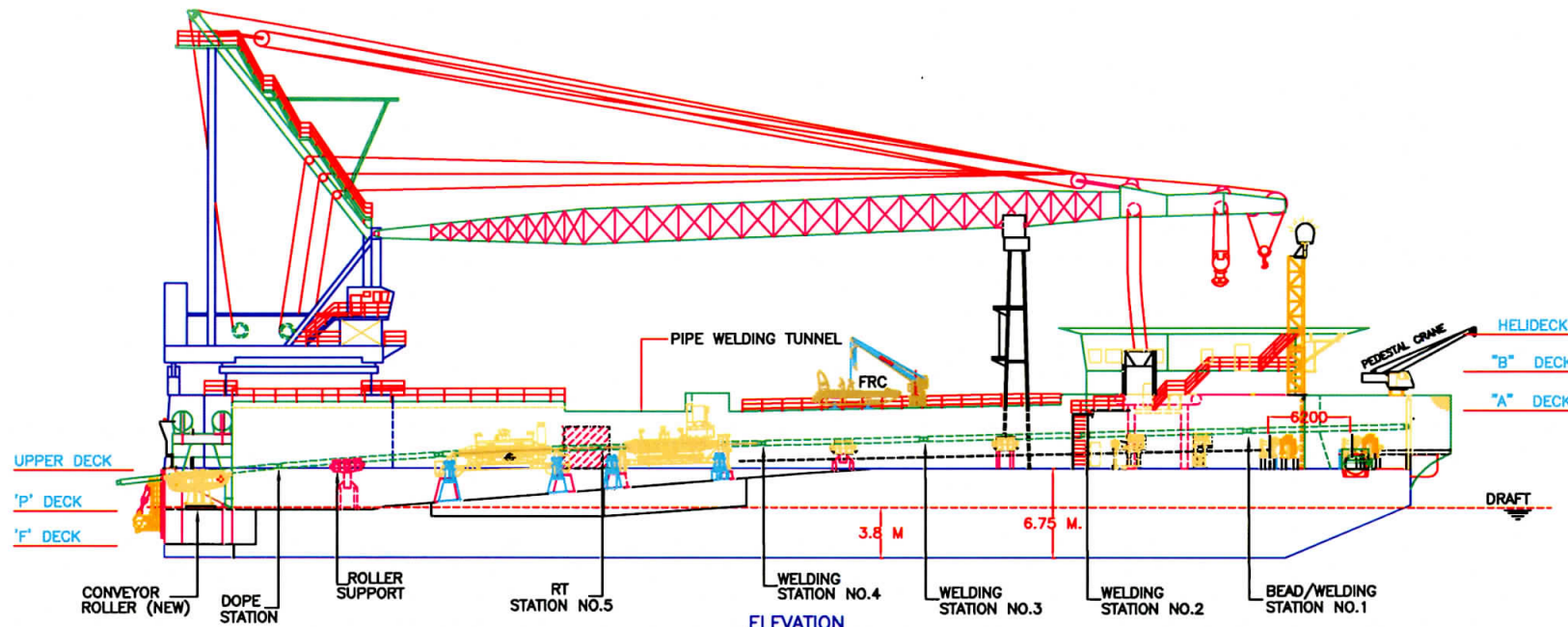
ELEVATION (OTHER DETAILS ARE NOT SHOWN)
