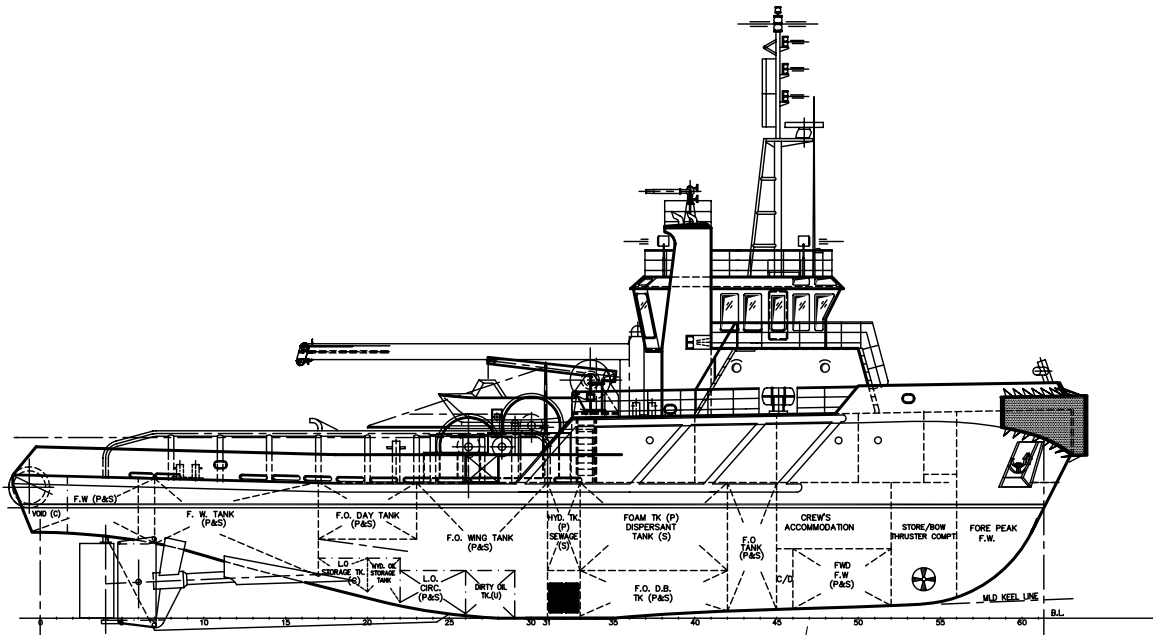
OUTBOARD PROFILE
