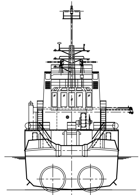
STERN VIEW
