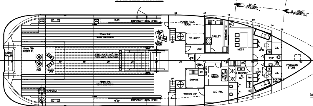
MAIN DECK
