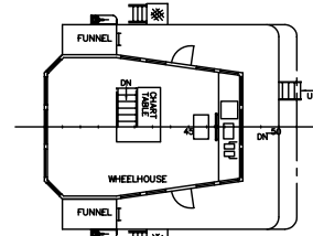
WHEELHOUSE DECK
