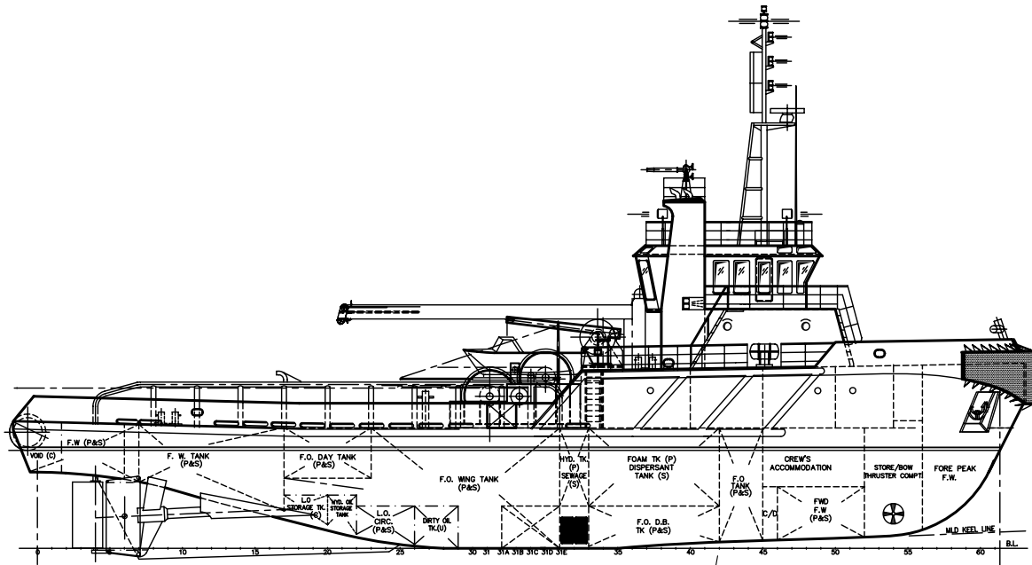
OUTBOARD PROFILE
