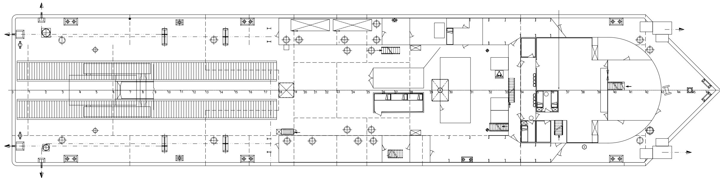
MAIN DECK PLAN
