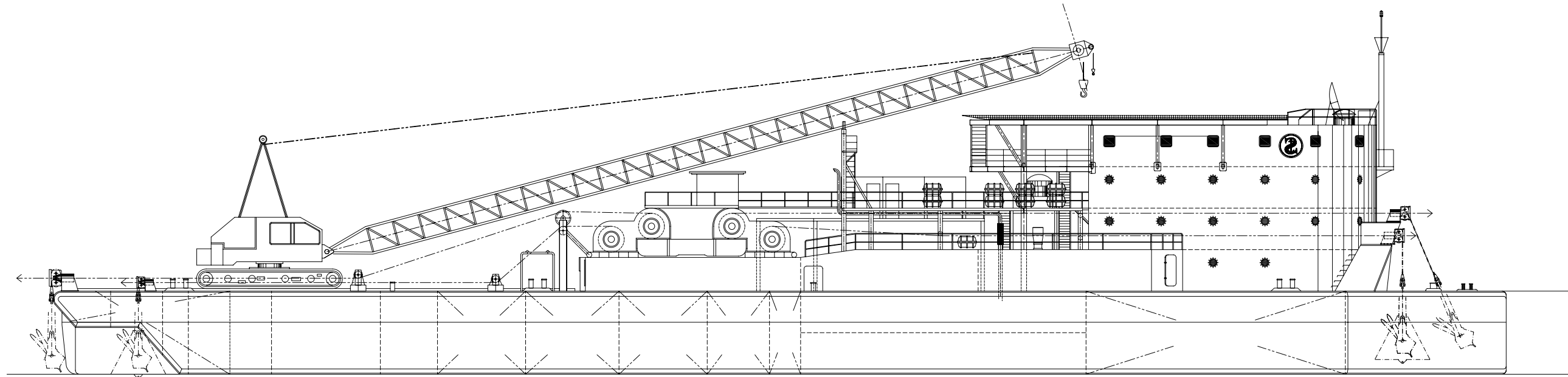
OUTBOARD PROFILE
